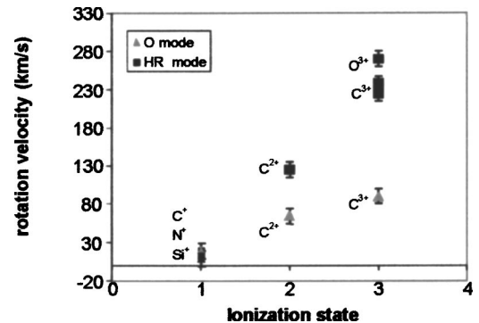
FIG. 6. Doppler ion rotation velocity vs impurity ionization state for both O and HR mode plasmas.
